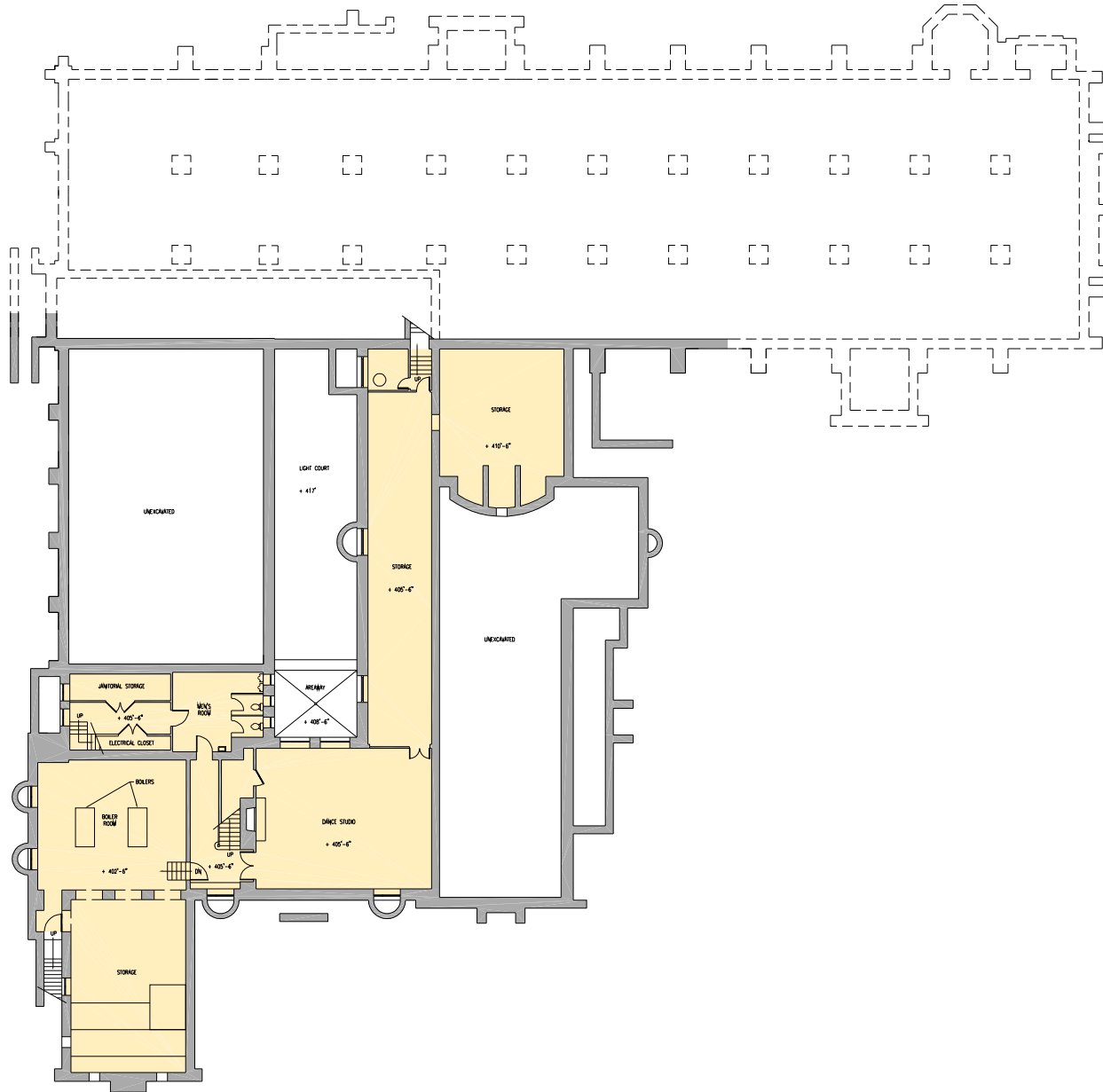
Existing Basement Plan
